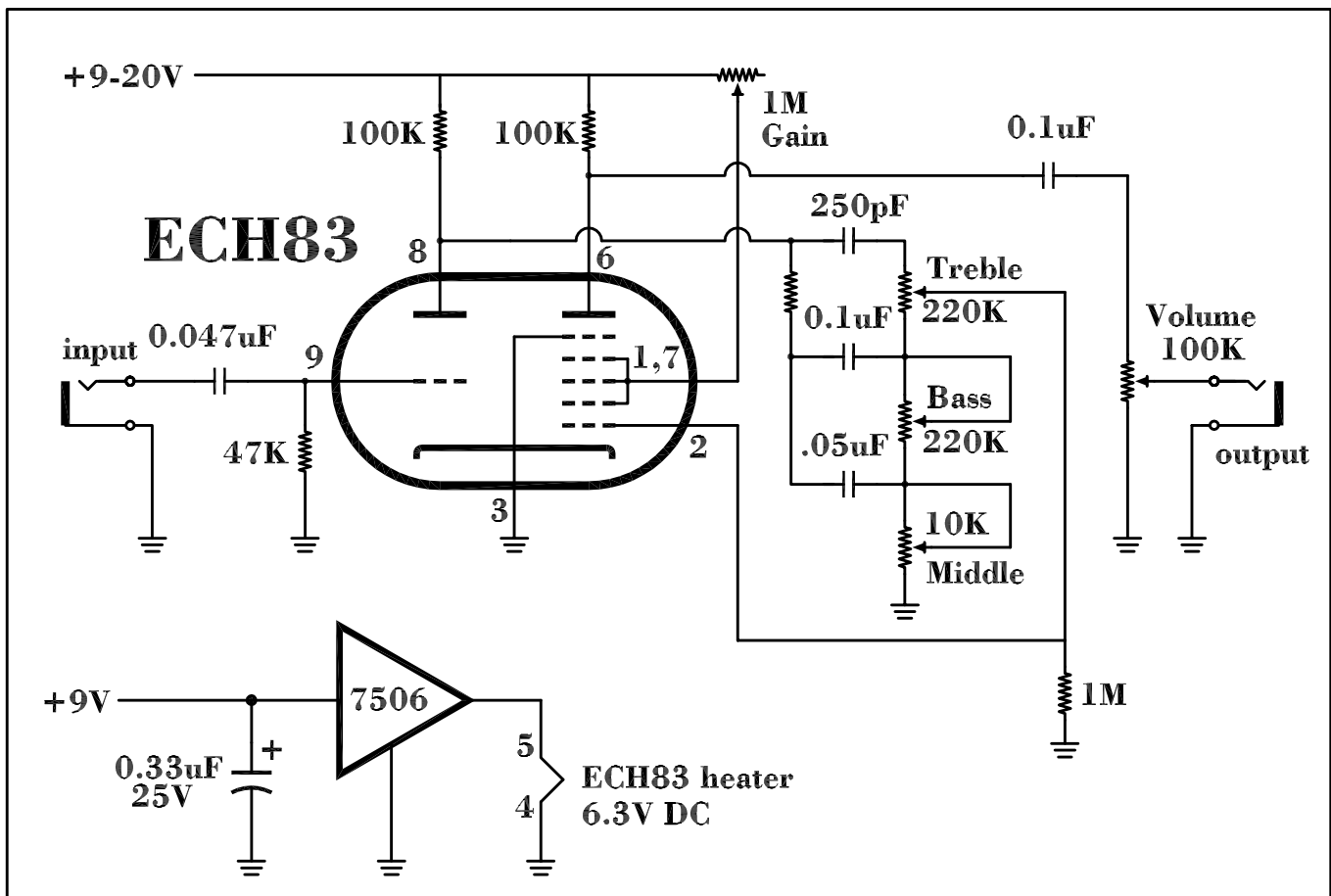
ECH83 guitar preamplifier with tone stack
