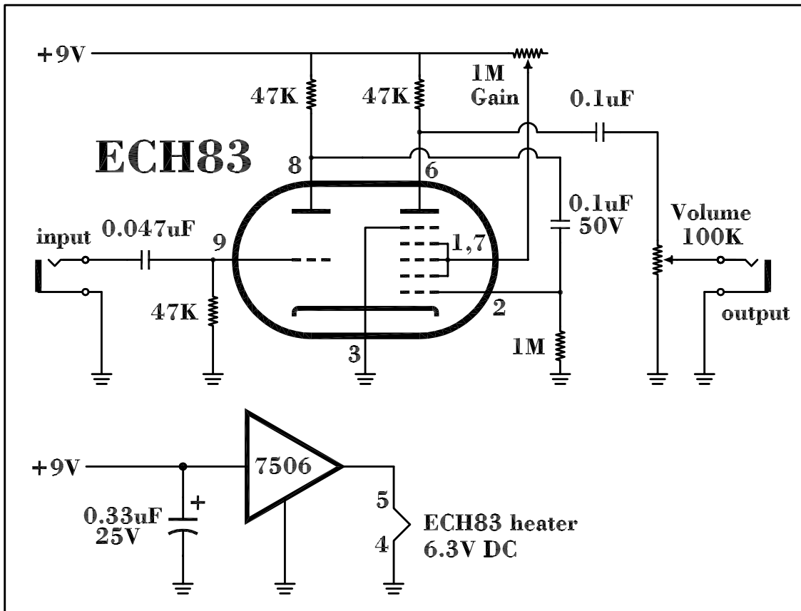
ECH83 guitar preamplifier - simple
